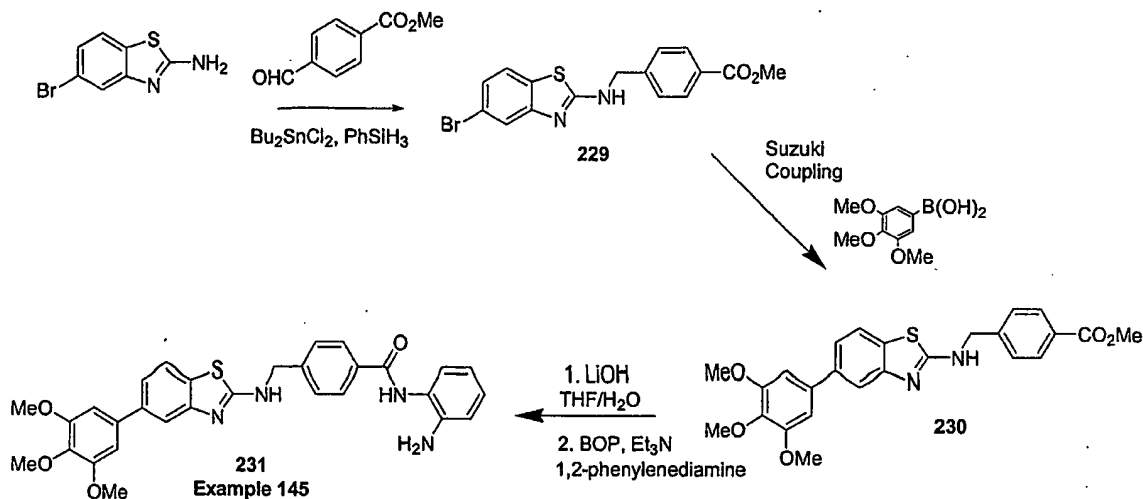
Scheme 34
